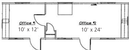
Mobile Office 40' x 10' (36' x 10' box size)
