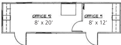
Mobile Office 36' x 8' (32' x 8' box size)
