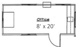
Mobile Office 24' x 8' (20' x 8' box size)
