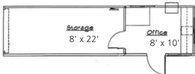
Office Storage Combo 36' x 8' (32' x 8' box size)
