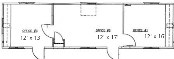
Mobile Office 50' x 12' (46' x 12' box size)
