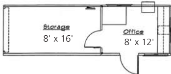
Office Storage Combo 32' x 8' (28' x 8' box size)
